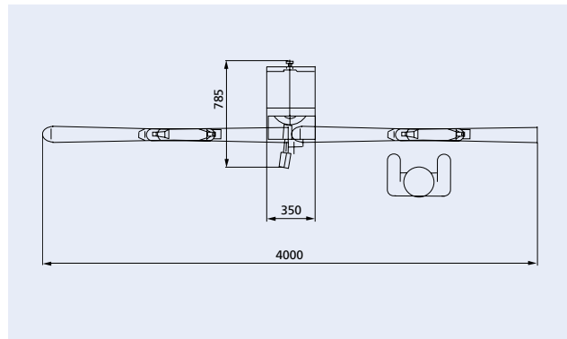
Layout KSM-F
