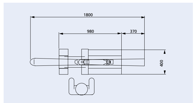
Grundriss DIATRONIC Pro
